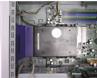
Air Duct joint Thermal module (TMA)
