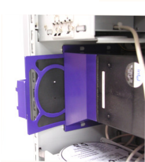
Cleanable Dust Filter
