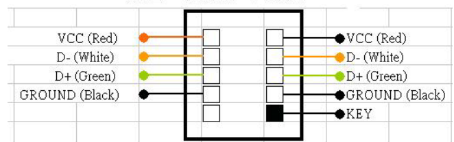
USB Cable Pinout
