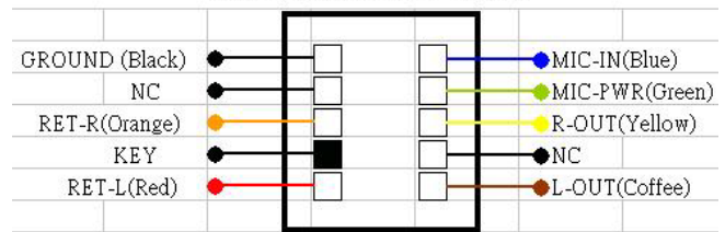
AUDIO Cable Pinout
