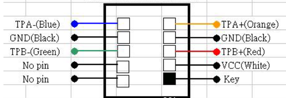
1394 cable connector
